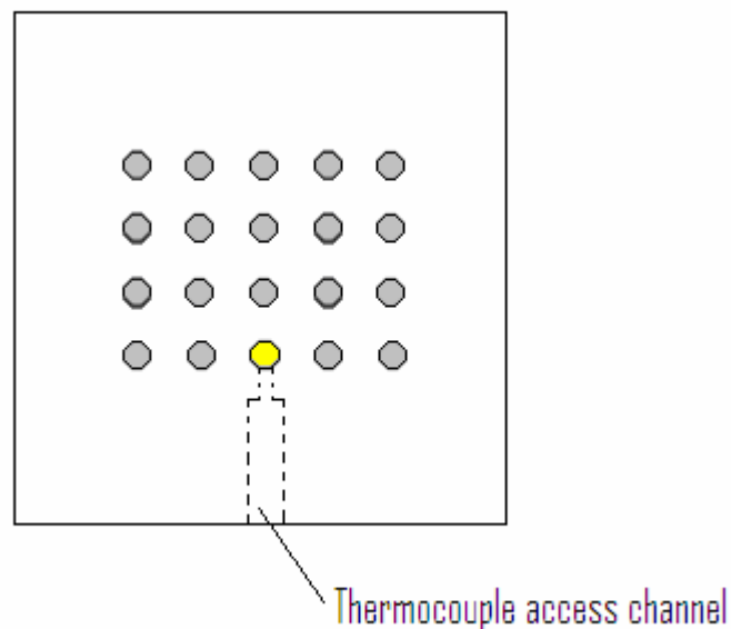
Fig. 1 SBT 0.8mm contact test arrangement
