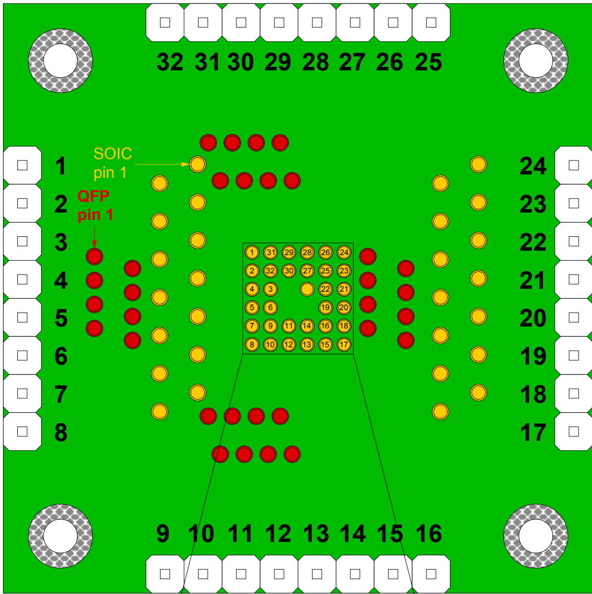
Top View (x-ray)
