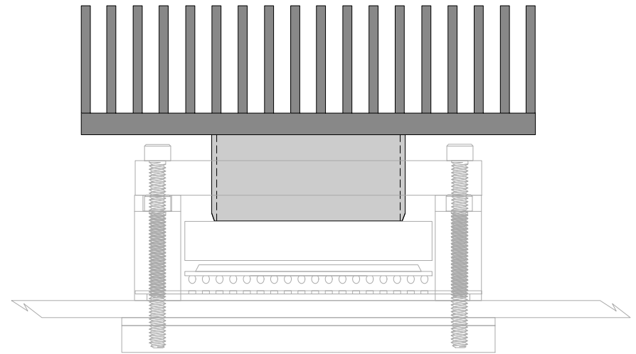
Socket Assembly(not to scale)
