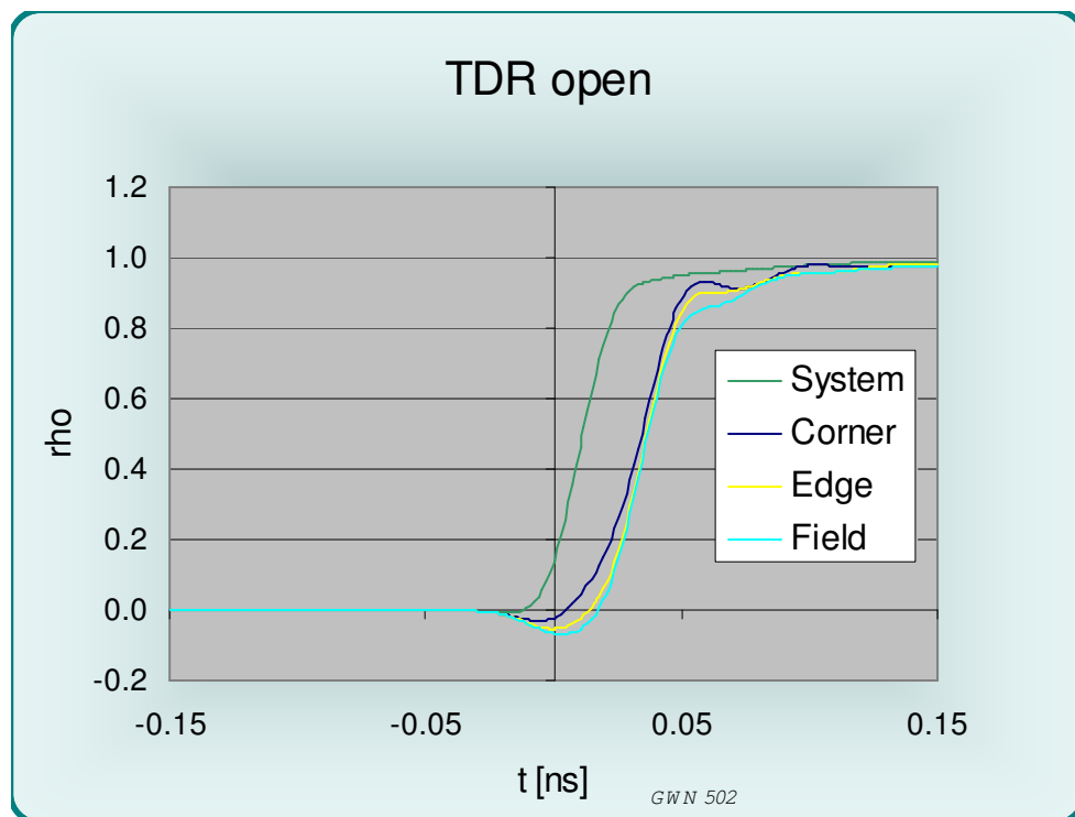
Figure 5 TDR signal from an OPEN circuited SBT test socket
