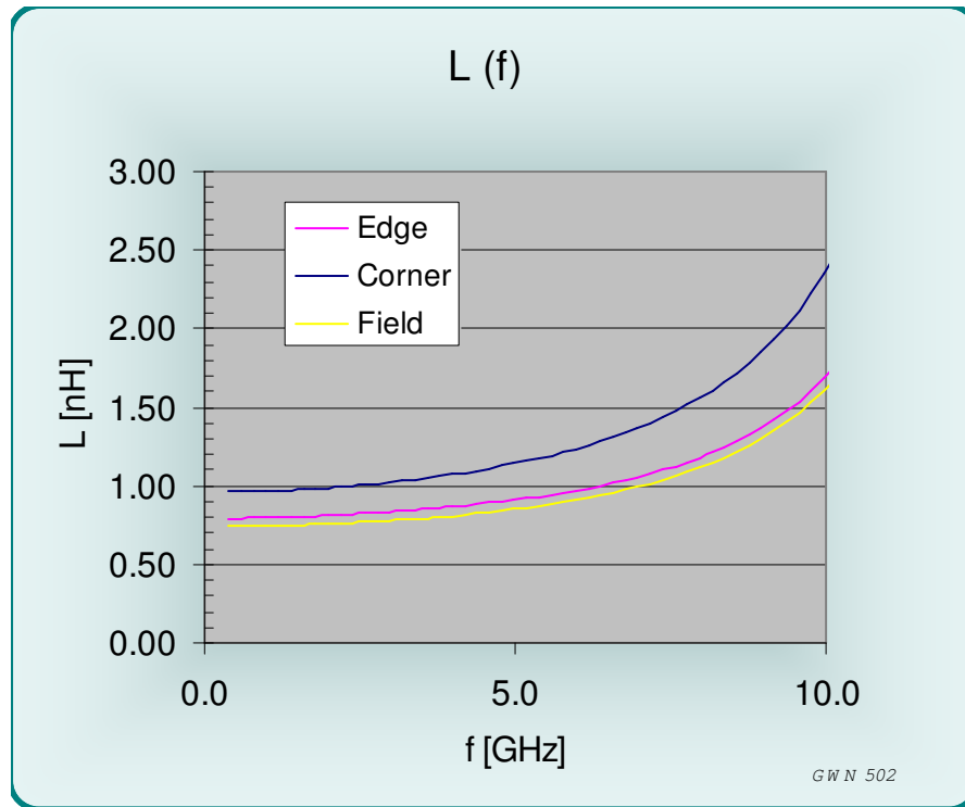
Figure 15 L(f) for the SBT test socket
