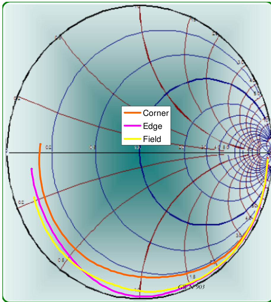
Figure 12 Reflections from the open circuited SBT test socket
