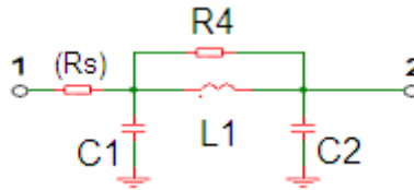
Figure 30 Lumped element SPICE model
