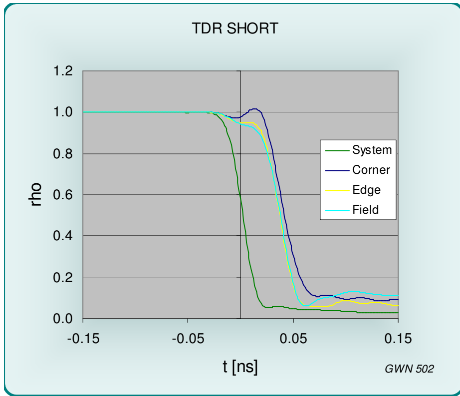
Figure 6 TDR signal from a SHORT circuited SBT test socket
