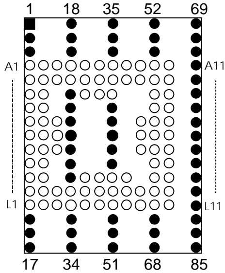
Top View-PGA(Alpha/Numeric)
