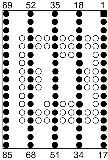
Bottom View-Base
