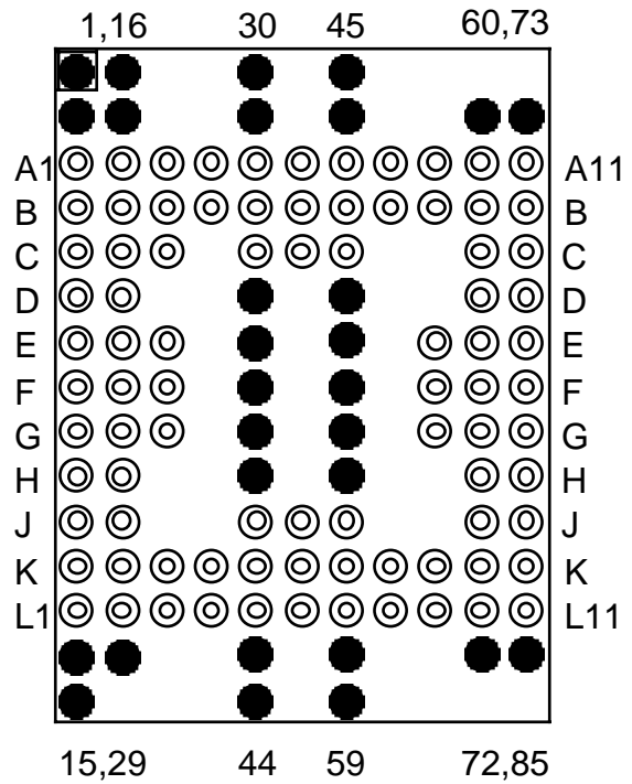
Top View- PGA
