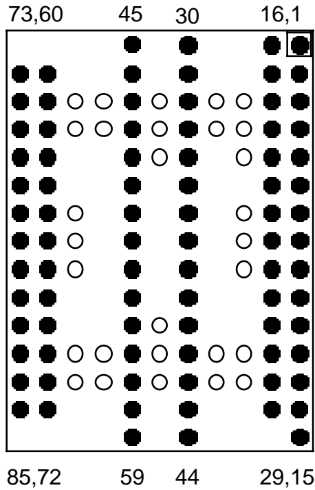
Bottom View- Base
