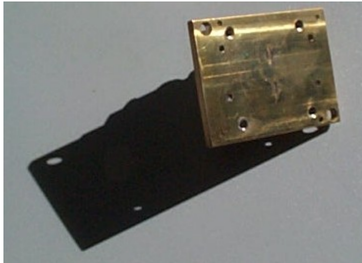
Figure 1 P-P152A spring probe base plate example
