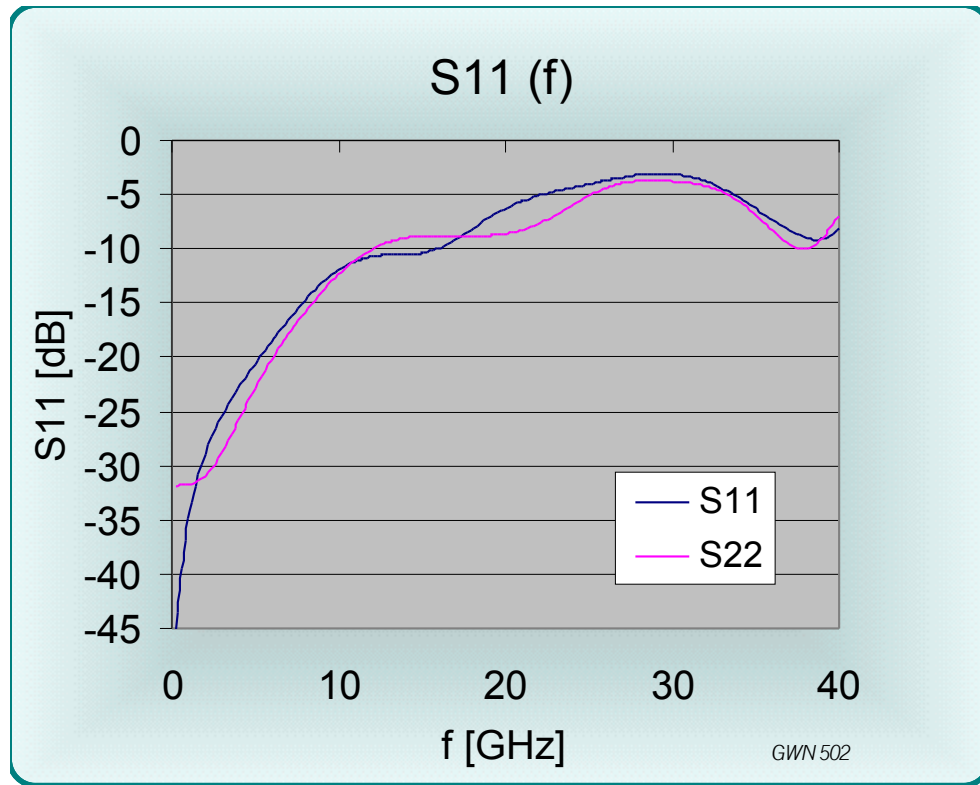
Figure 25 S11 magnitude (f) for the thru measurements into a 50 Ohm probe
