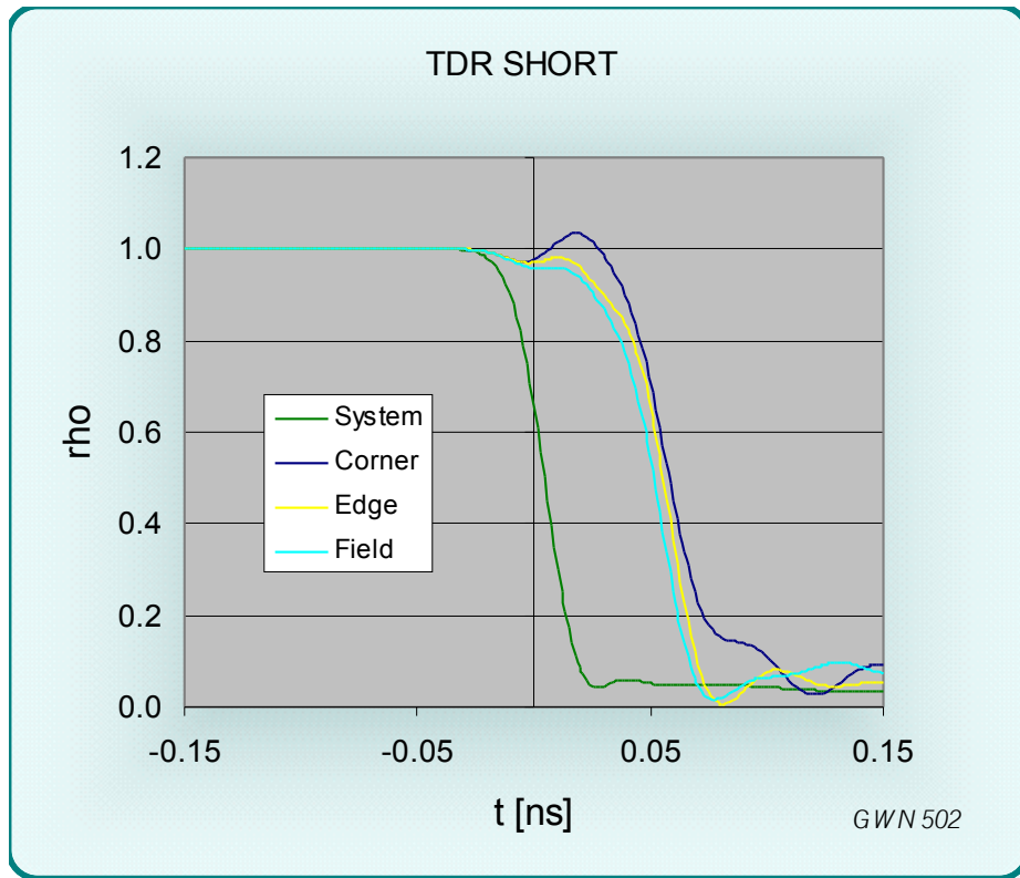
Figure 6 TDR signal from a SHORT circuited P-P152A array
