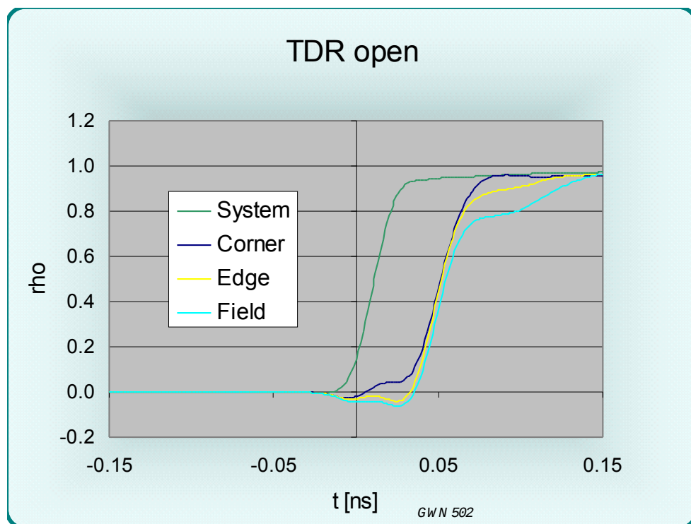
Figure 5 TDR signal from an OPEN circuited P-P152A array
