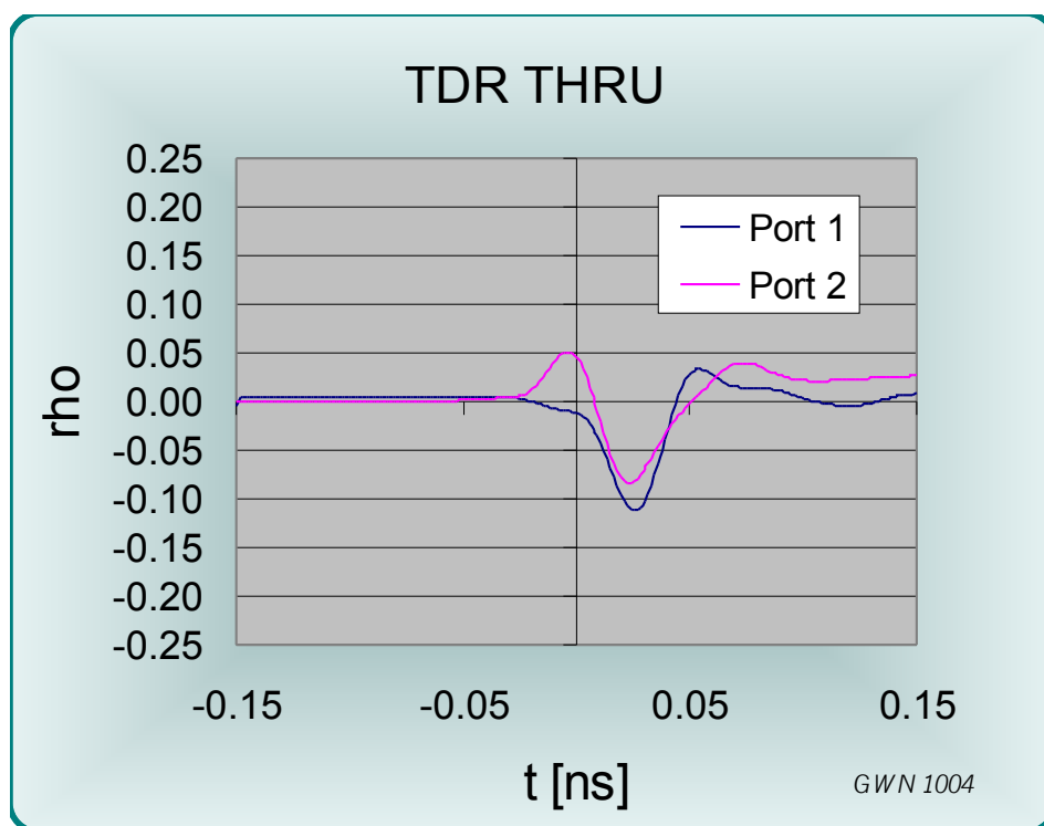
Figure 21 TDR through DUT into a terminated probe
