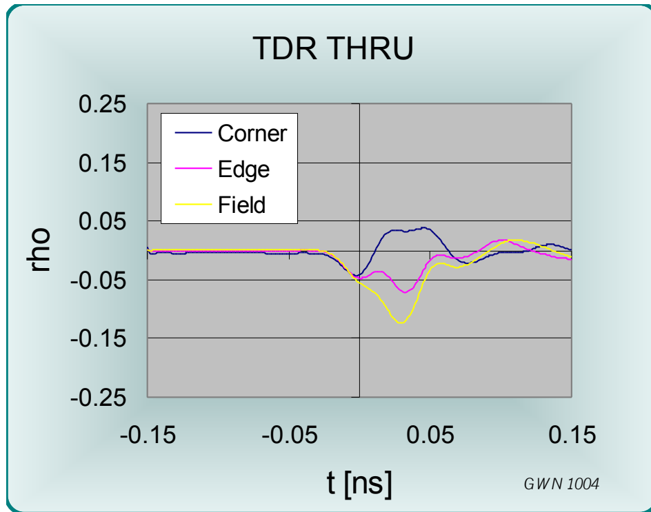
Figure 7 TDR measurement into a 50 Ohm probe
