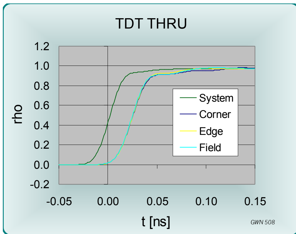
Figure 8 TDT measurement
