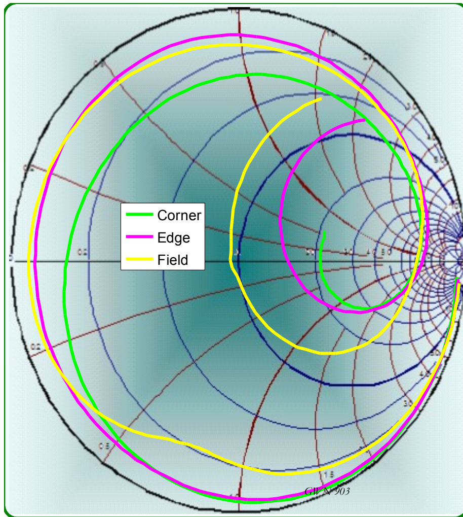
Figure 12 Reflections from the open circuited P-P152A array
