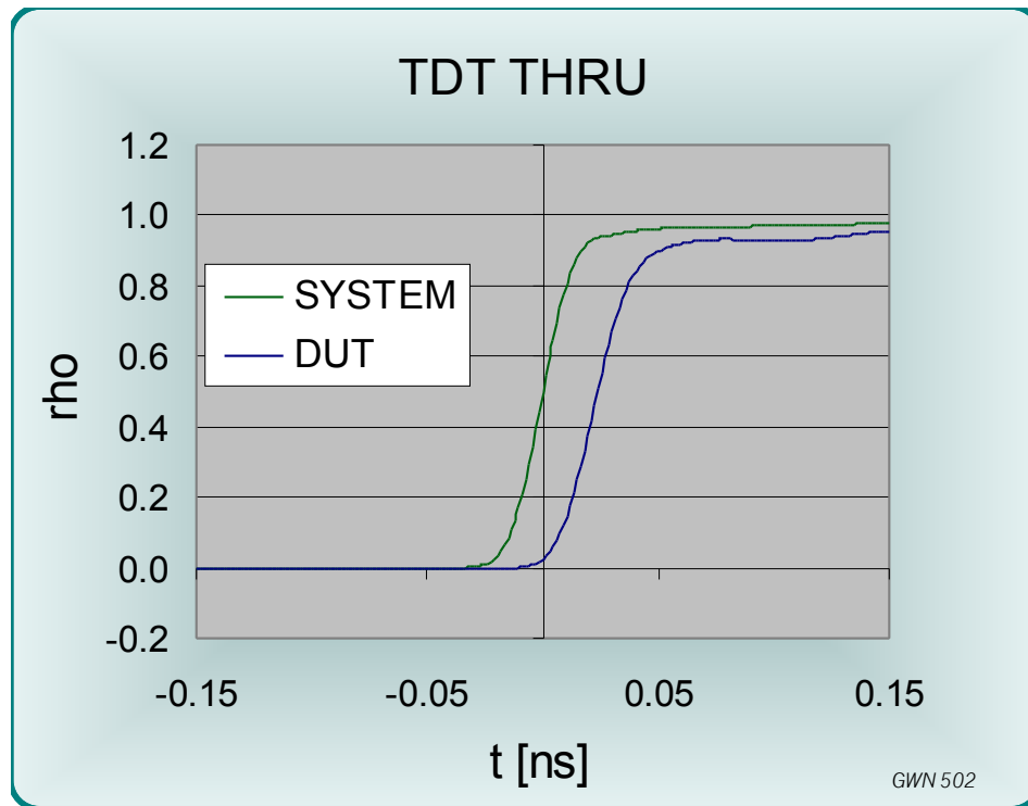
Figure 22 TDT measurement
