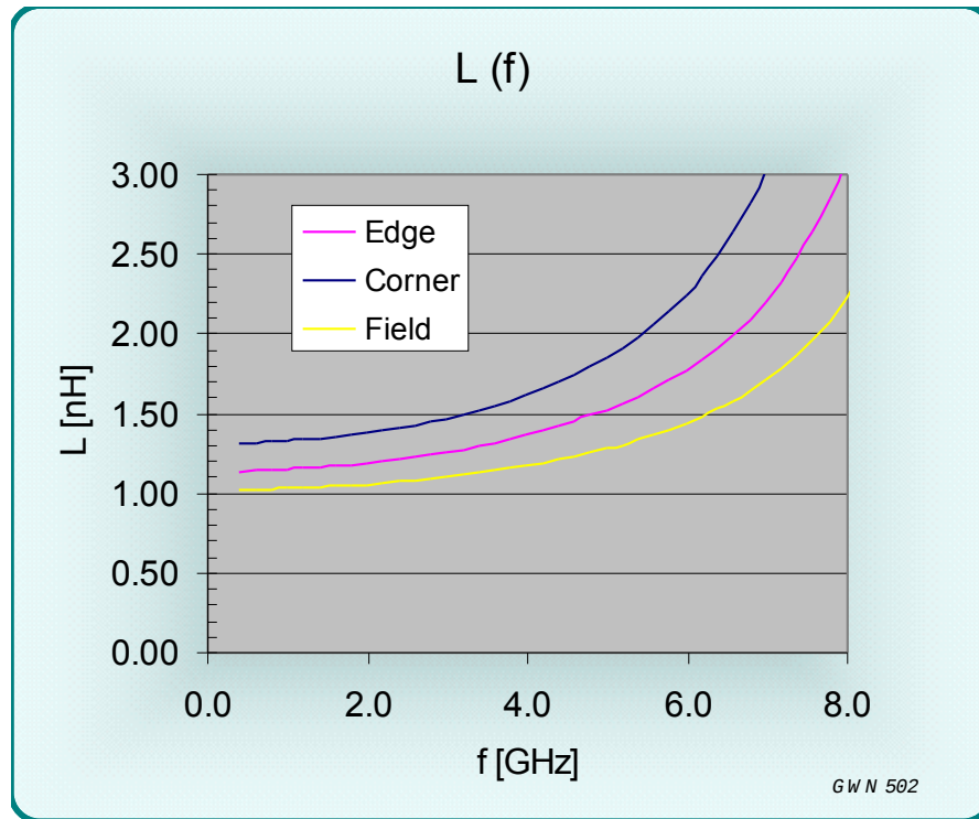
Figure 15 L(f) for the P-P152A array
