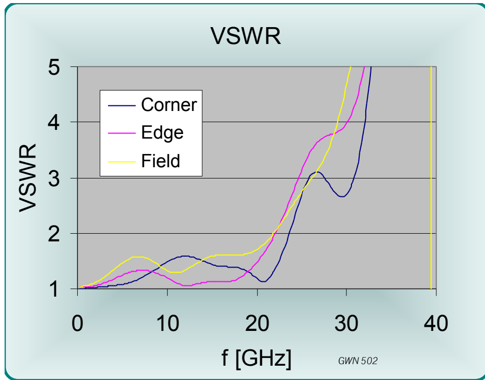
Figure 20 Standing wave ratio VSWR (f) [1 / div.]
