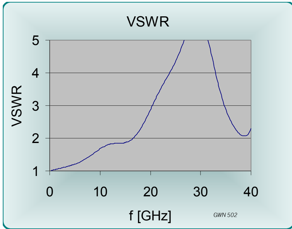
Figure 26 Standing wave ratio VSWR (f) [1 / div.]
