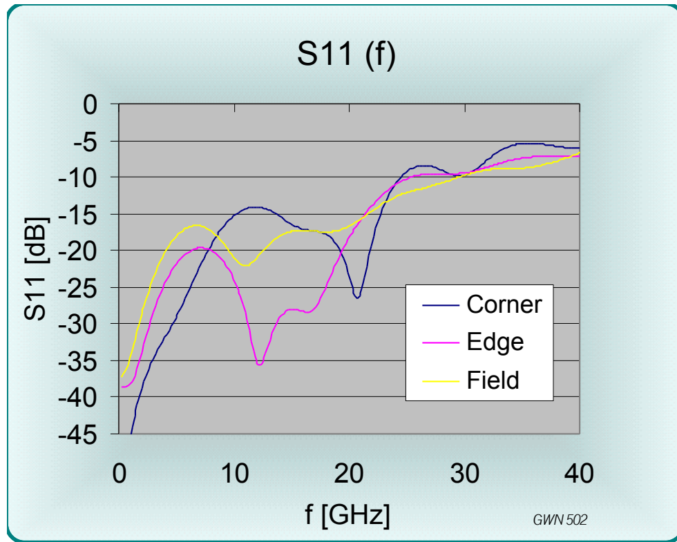
Figure 19 S11 magnitude (f) for the thru measurement into a 50 Ohm probe
