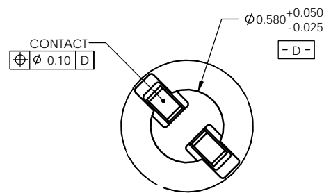
DETAIL B 170X SCALE 4:1
