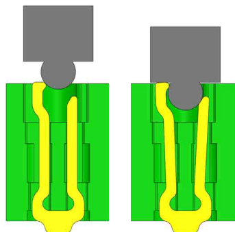
Cross section view of test socket and package.
