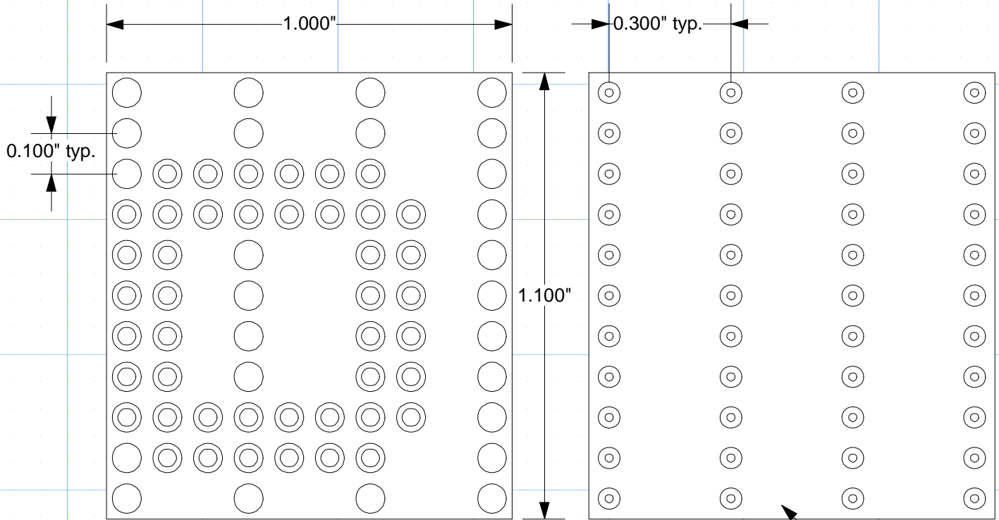
Bottom View (only male pins shown for drawing clarity)
