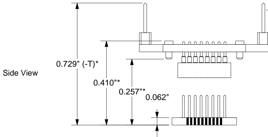
44 Pin Surface-Mountable Foot (QFE44SB)
