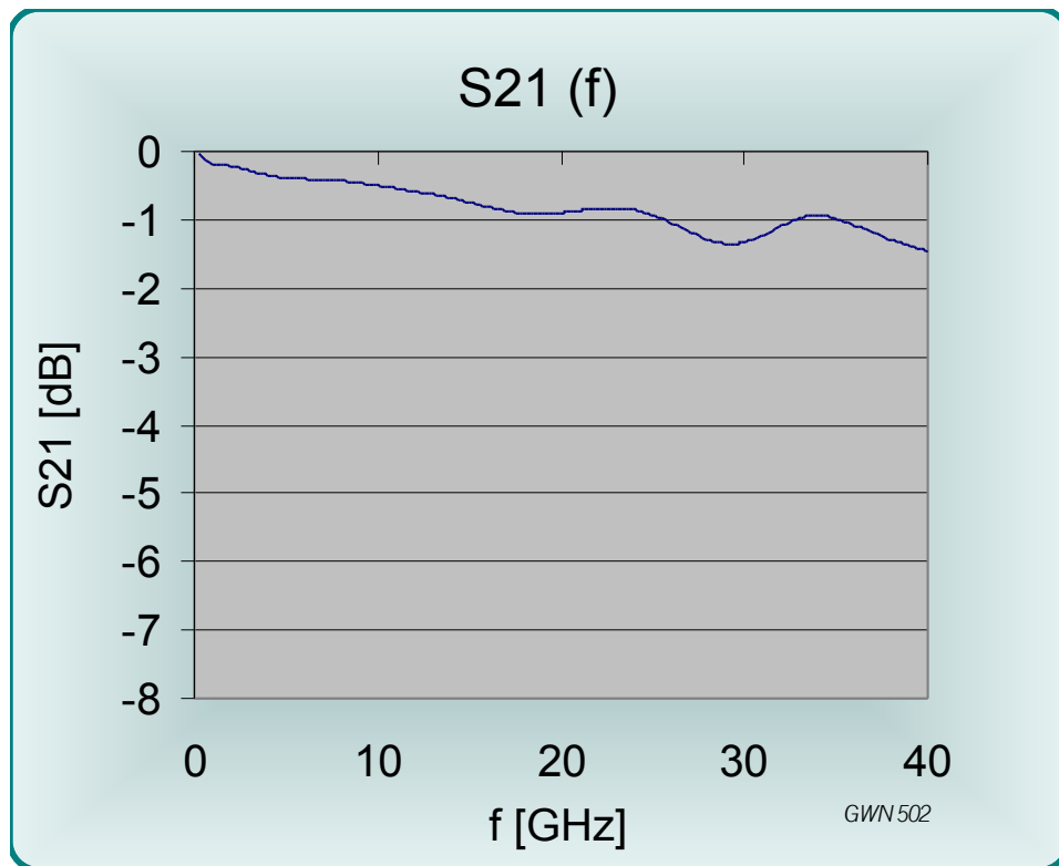
Figure 23 Insertion loss S21 (f)
