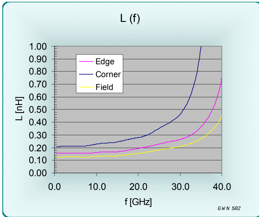
Figure 15 L(f) for the SMP contacts (0.6mm height)
