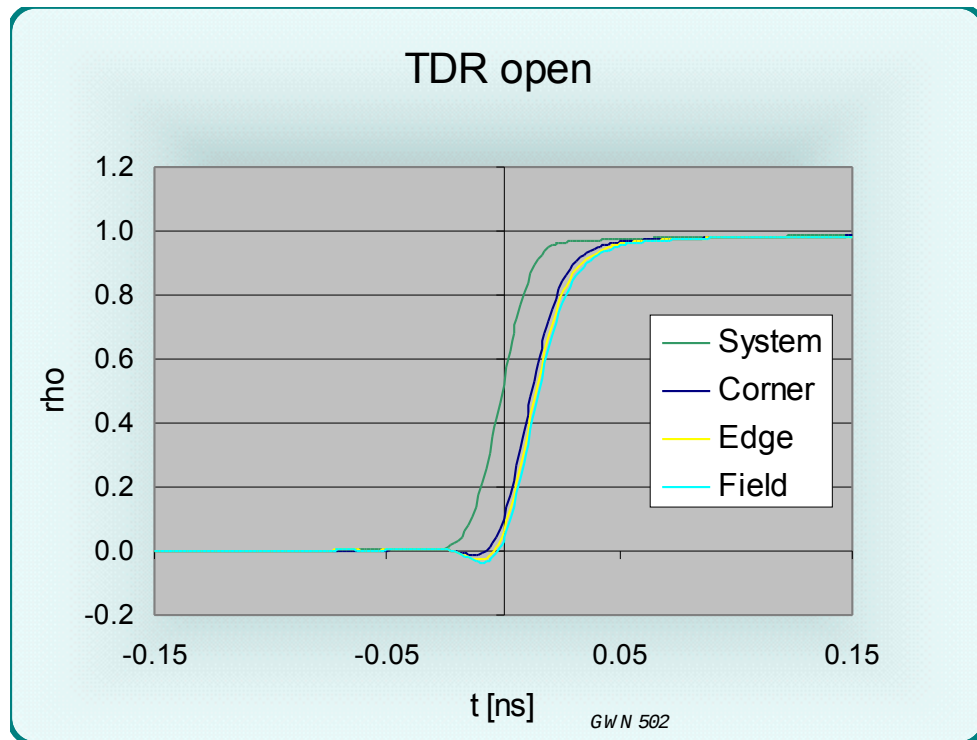
Figure 5 TDR signal from an OPEN circuited SMP contacts (0.6mm height)
