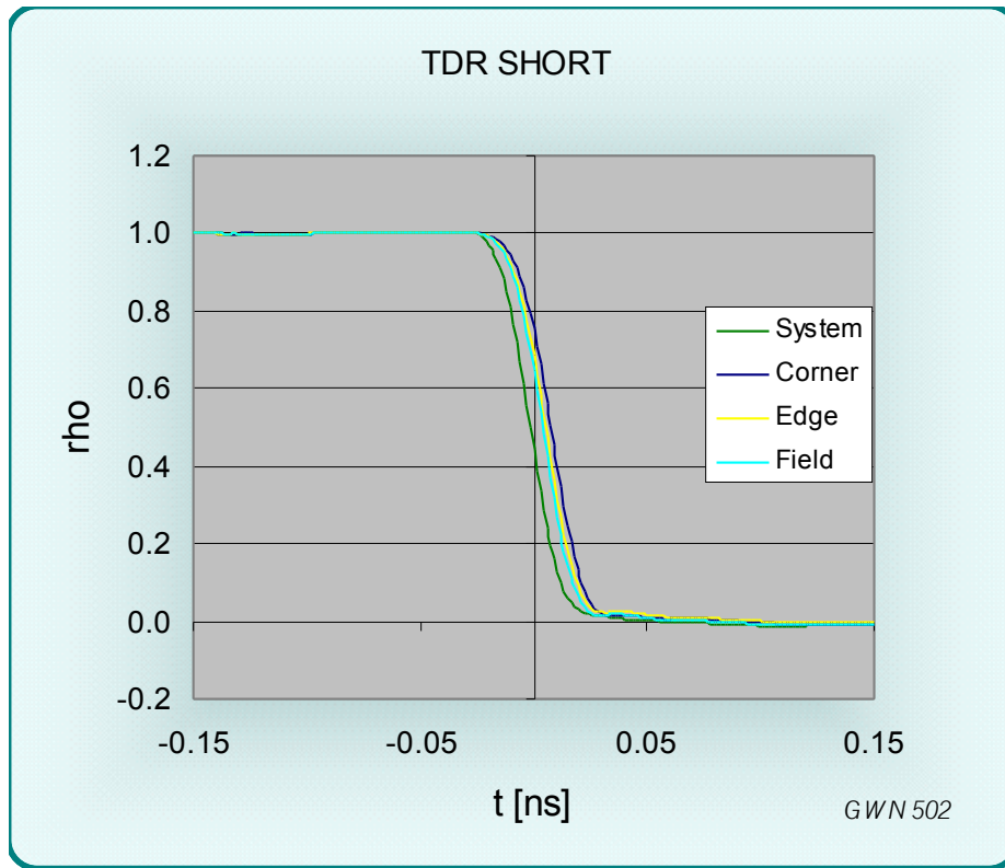
Figure 6 TDR signal from a SHORT circuited SMP contacts (0.6mm height)
