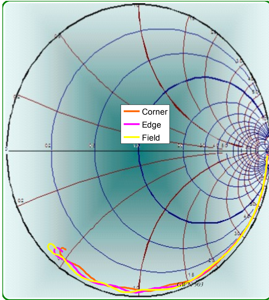
Figure 12 Reflections from the open circuited SMP contacts (0.6mm height)
