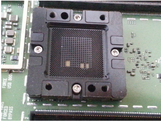
Above Near Zero Footprint Spring Pin Socket mounted to an evaluation board
