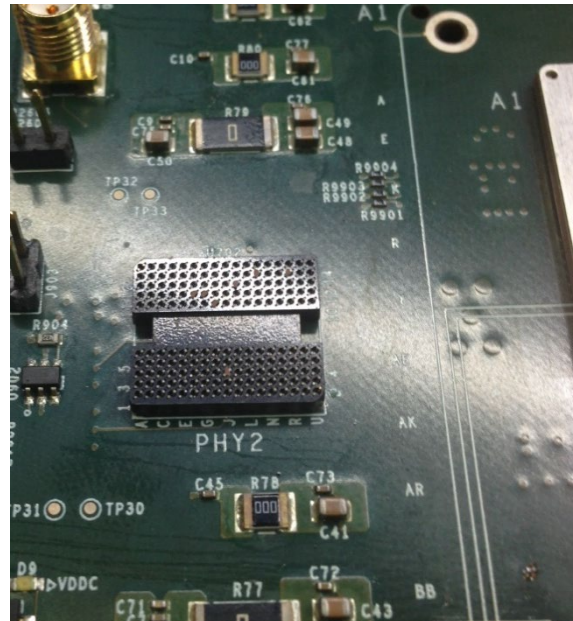
Above Grypper on a validation PCB for GDDR5 Device
