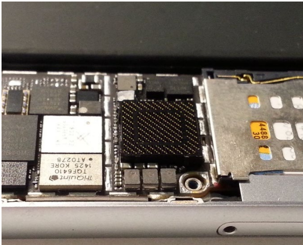
Above Grypper installed into a phone – Grypper socket is the same size as the device so it fits into the exact space as the device
