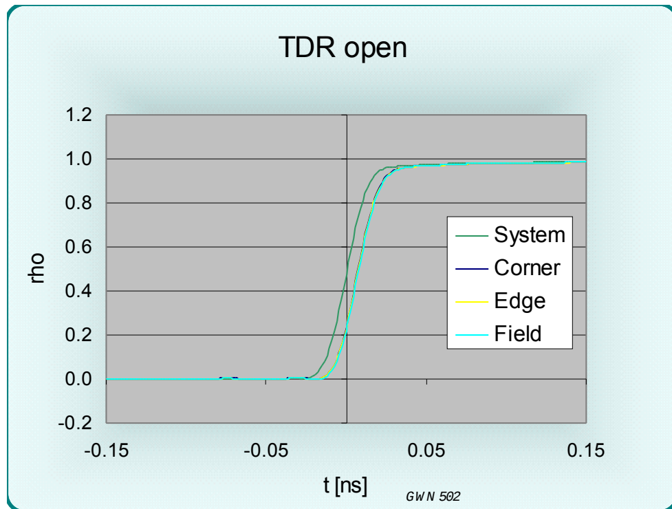
Figure 5 TDR signal from an OPEN circuited 0.5mm BGA test socket
