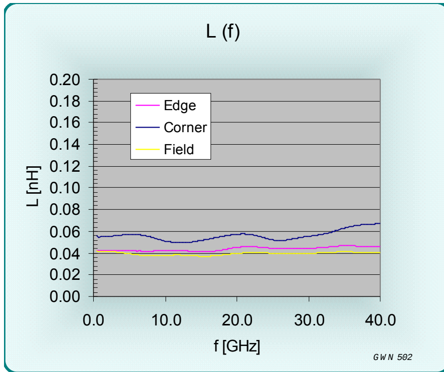
Figure 15 L(f) for the 0.5mm BGA test socket
