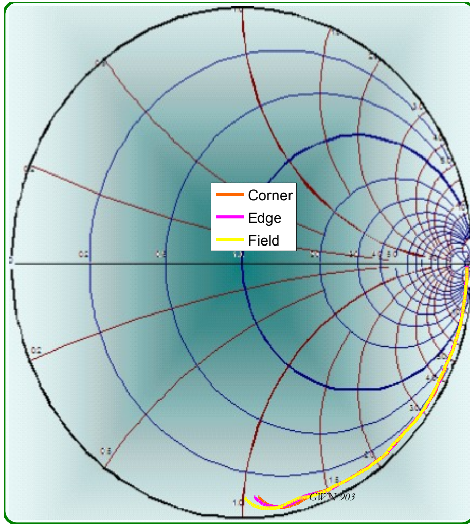
Figure 12 Reflections from the open circuited 0.5mm BGA test socket
