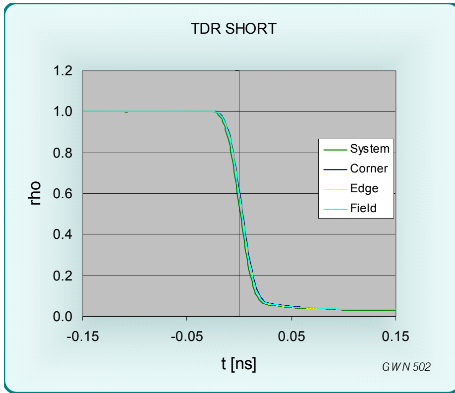
Figure 6 TDR signal from a SHORT circuited 0.5mm BGA test socket
