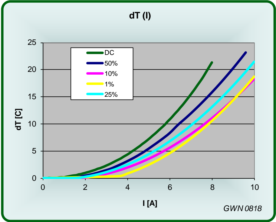
Figure 9 Temperature rise as a function of drive current*
