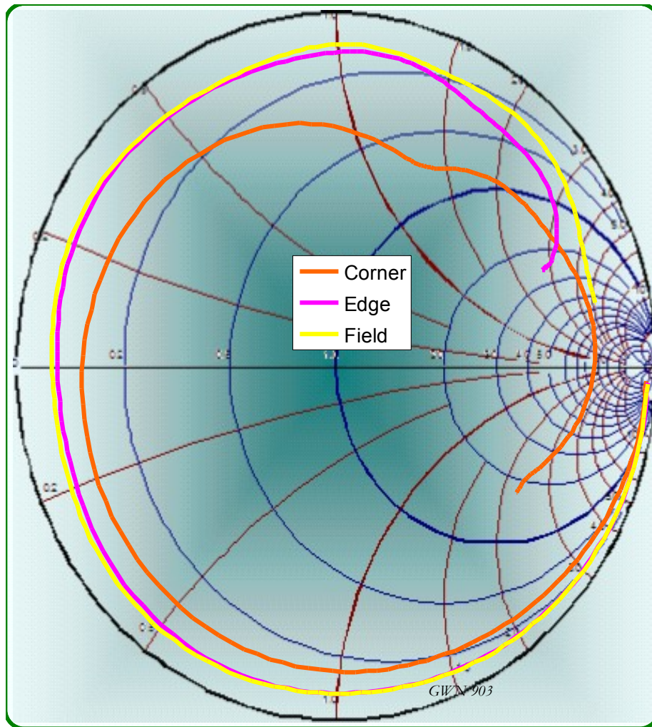
Figure 12 Reflections from the open circuited P-P204A test socket
