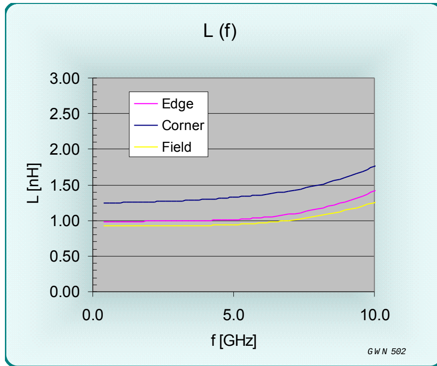
Figure 15 L(f) for the P-P204A test socket
