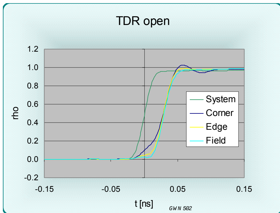
Figure 5 TDR signal from an OPEN circuited P-P204A test socket
