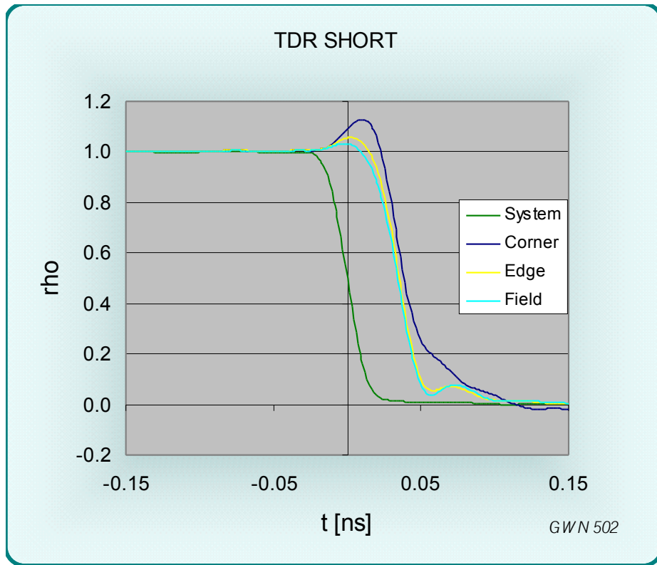
Figure 6 TDR signal from a SHORT circuited P-P204A test socket
