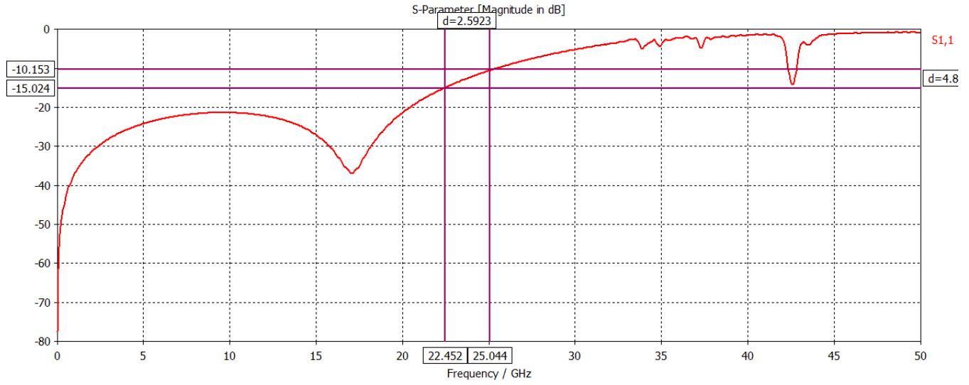
Fig. 3: Simulated Return Loss S1,1
