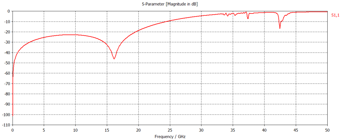
Fig. 3: Simulated Return Loss S 1,1
