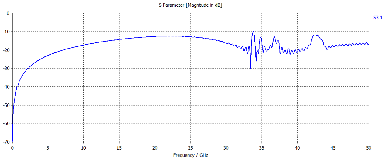
Fig.4 : Crosstalk. S31
