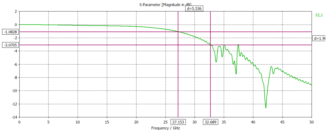
Fig. 2: Simulated Insertion loss
