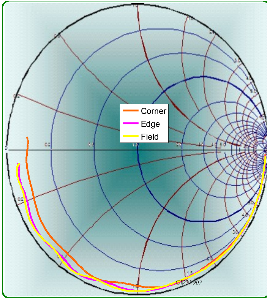
Figure 12 Reflections from the open circuited SMP contacts (1.0mm height)
