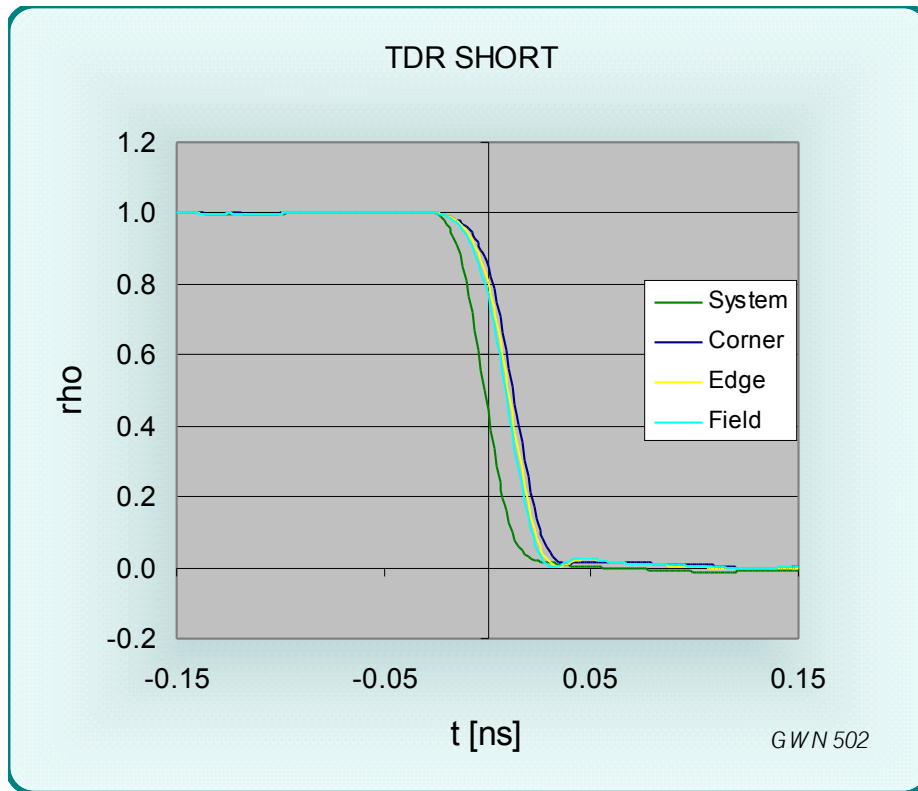
Figure 6 TDR signal from a SHORT circuited SMP (1.0mm height)
