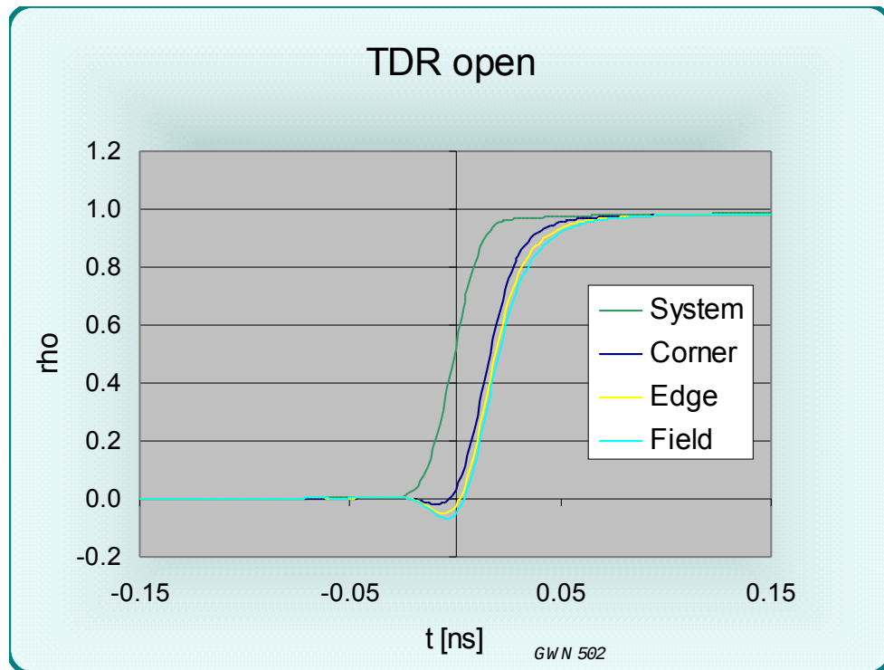
Figure 5 TDR signal from an OPEN circuited SMP contacts (1.0mm height)
