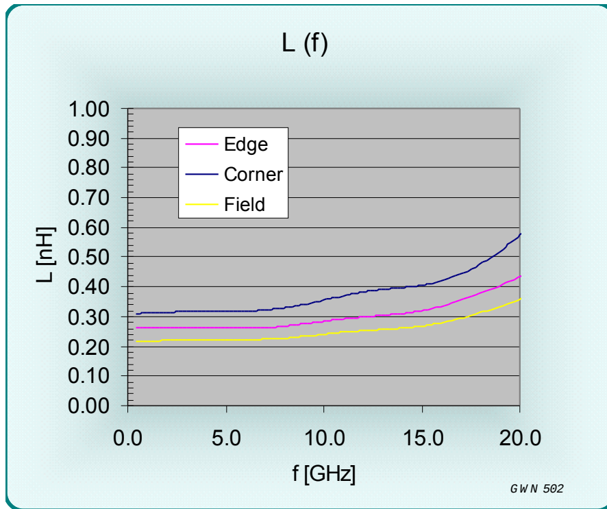
Figure 15 L(f) for the SMP (1.0mm height)
