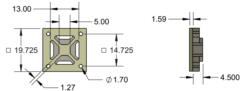
Insulation and Backing Plate
