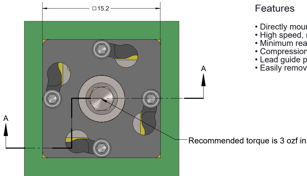
TOP VIEW
