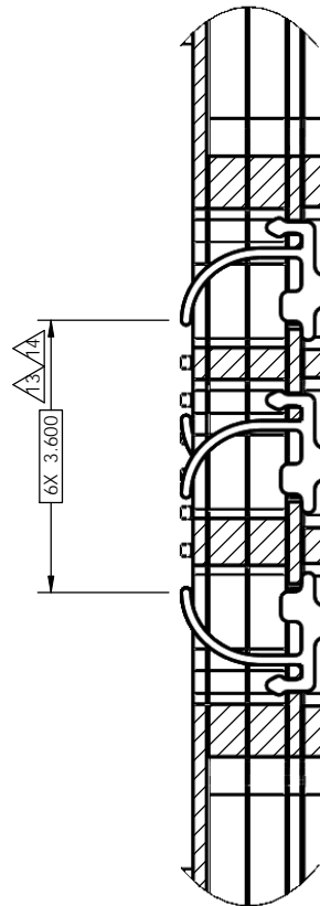
DETAIL D SCALE 3:1
