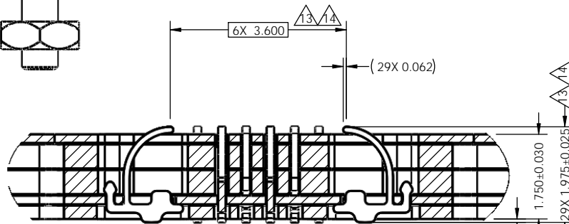
DETAIL C SCALE 3:1
