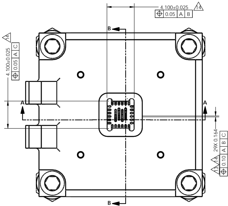
TOP VIEW W/O LID
