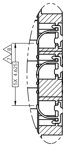
DETAIL D SCALE 2:1
