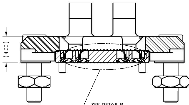
SEE DETAIL B SECTION A-A (ROTATED 90° CW)
