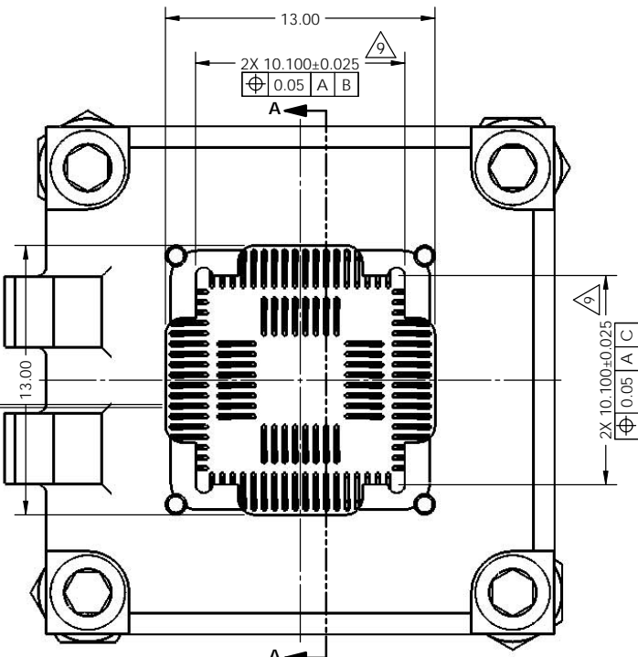
TOP VIEW W/O LID SCALE 3:2
