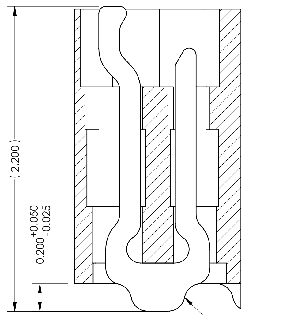
SECTION B-B Scale 10:1 (ROTATED 45° CW)
