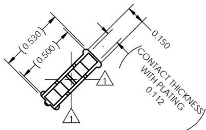
DETAIL C (221X) SCALE 8:1
