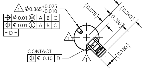
DETAIL B (221X) SCALE 8:1
