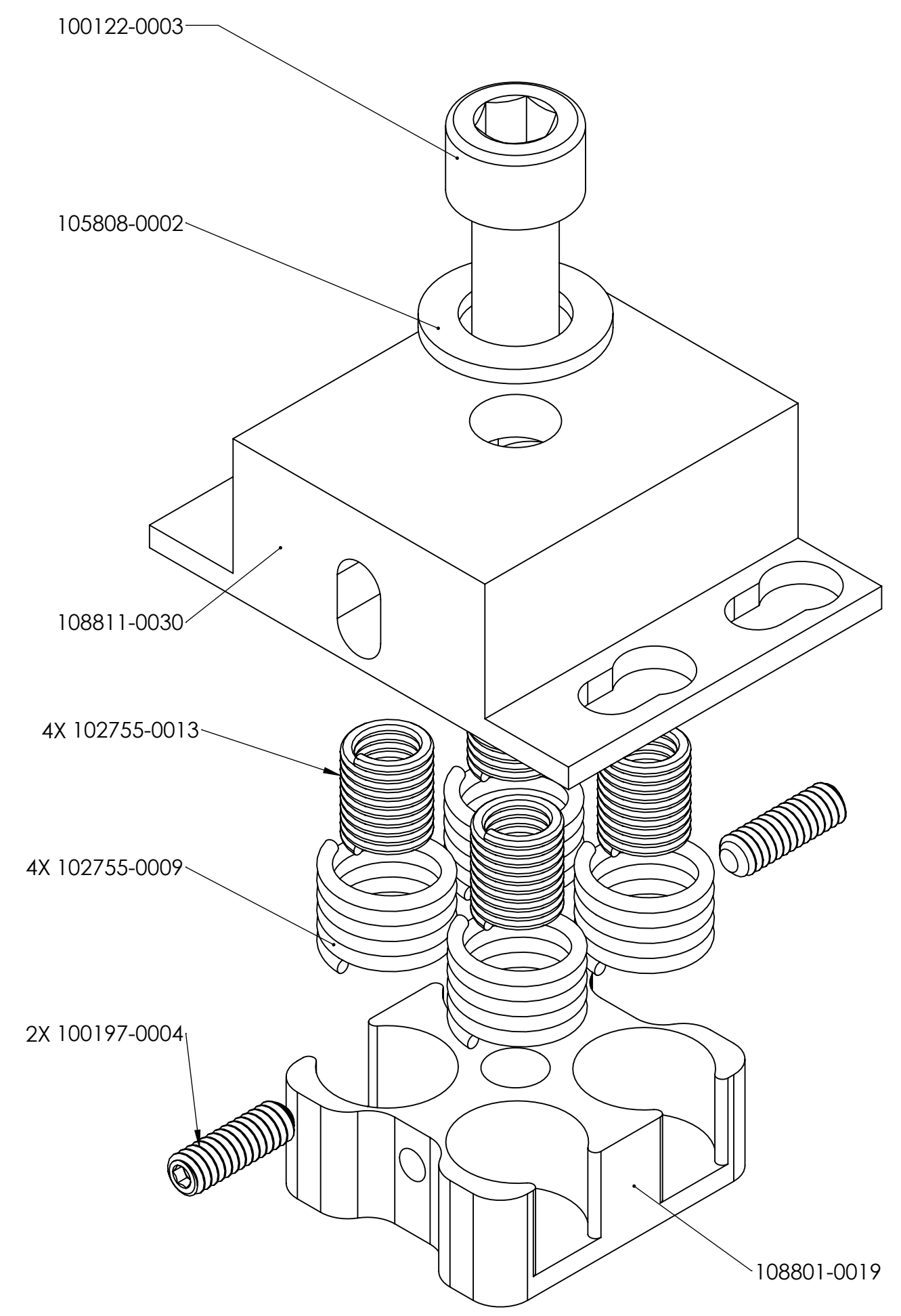
SLIDING LID ASSEMBLY 108810-0050
