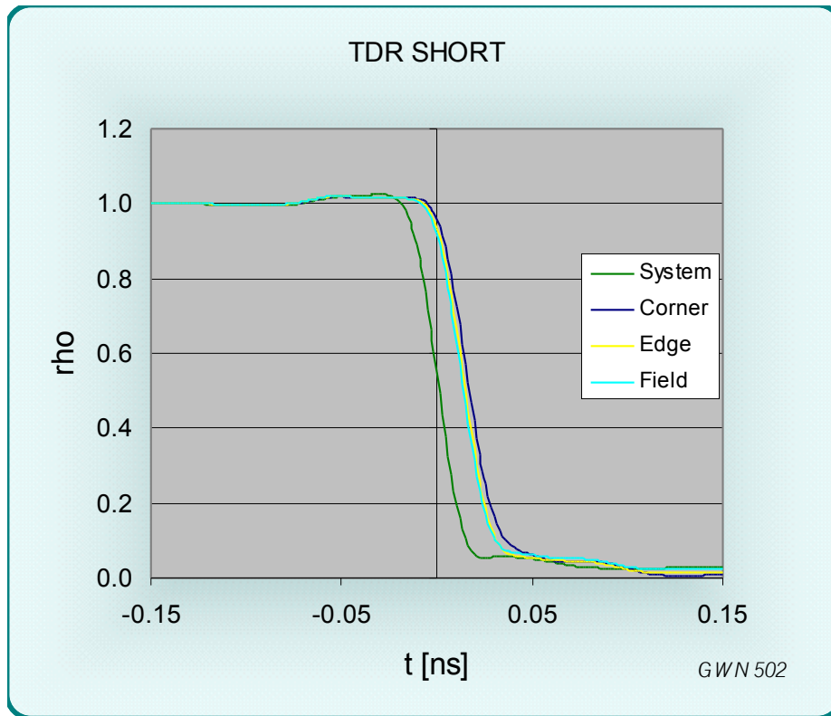
Figure 6 TDR signal from a SHORT circuited GR1279 test socket
