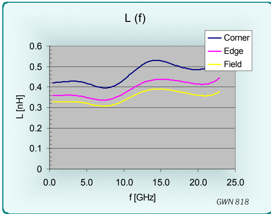
Figure 15 L(f) for the GR1279 test socket
