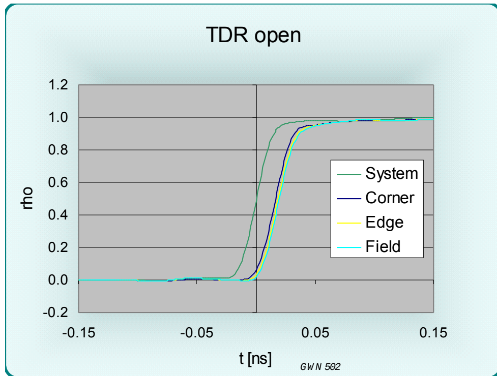
Figure 5 TDR signal from an OPEN circuited GR1279 test socket
