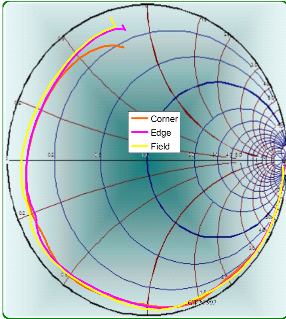
Figure 12 Reflections from the open circuited GR1279 test socket
