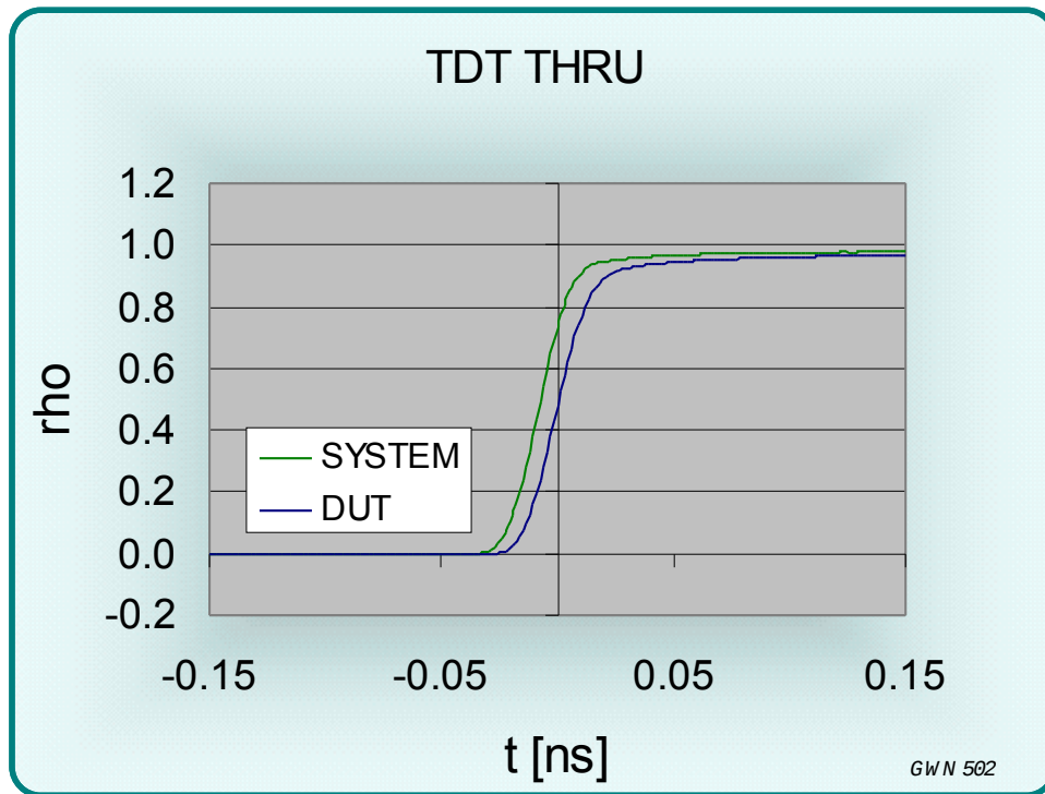
Figure 22 TDT measurement
