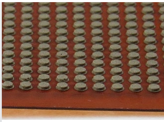
Array of Silver Buttons - Elastomer Matrix
