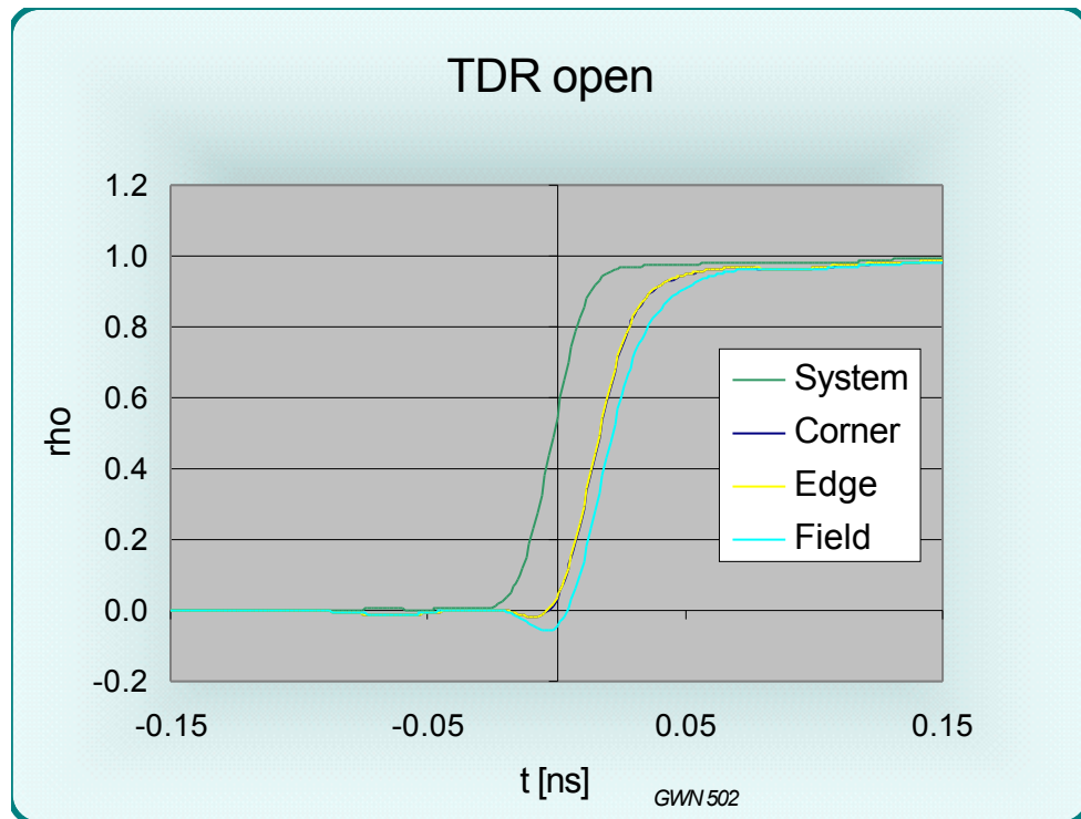
Figure 5 TDR signal from an OPEN circuited DUT test socket
