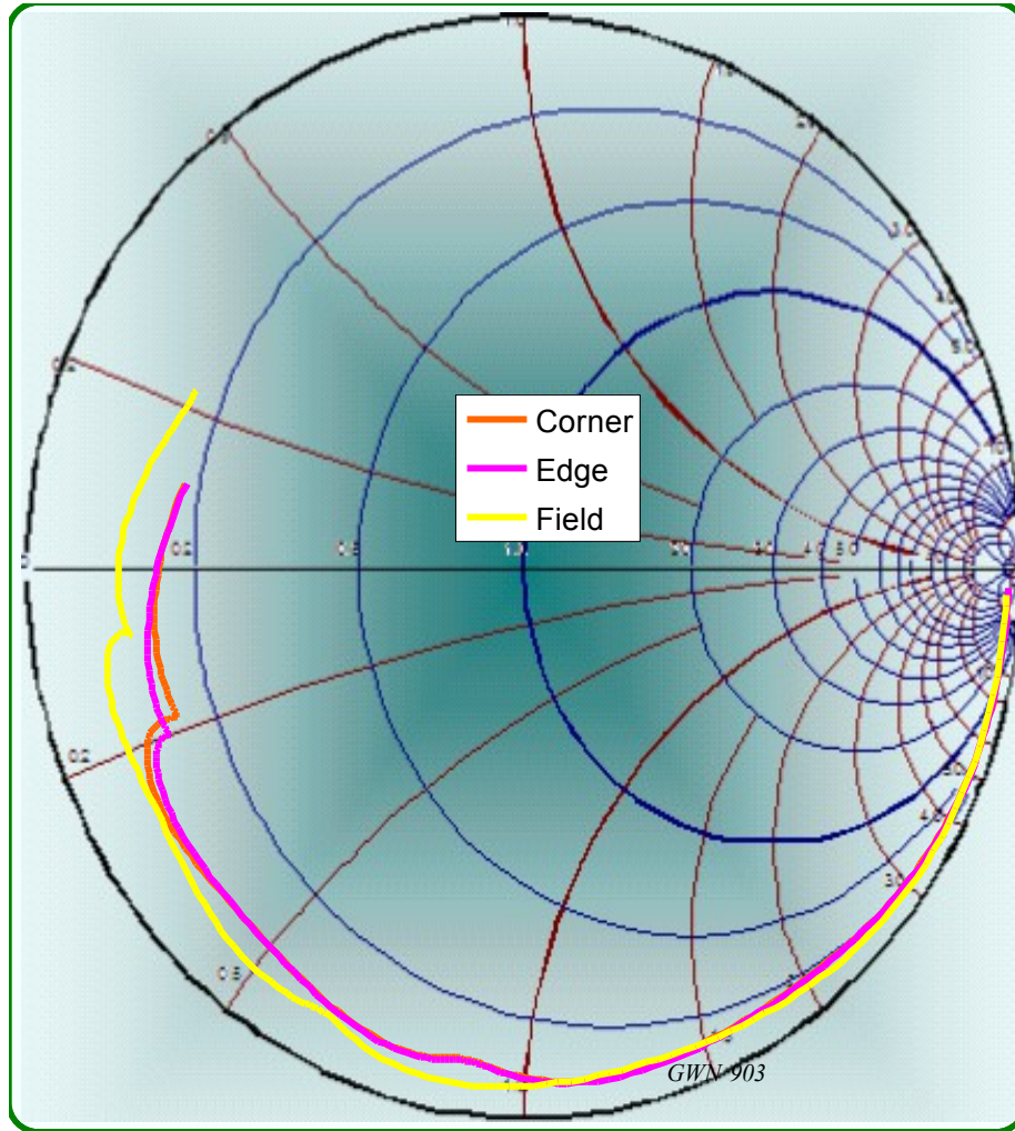
Figure 12 Reflections from the open circuited DUT test socket
