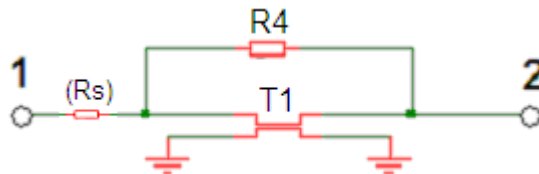
Figure 31 Transmission line model for the DUT test socket
