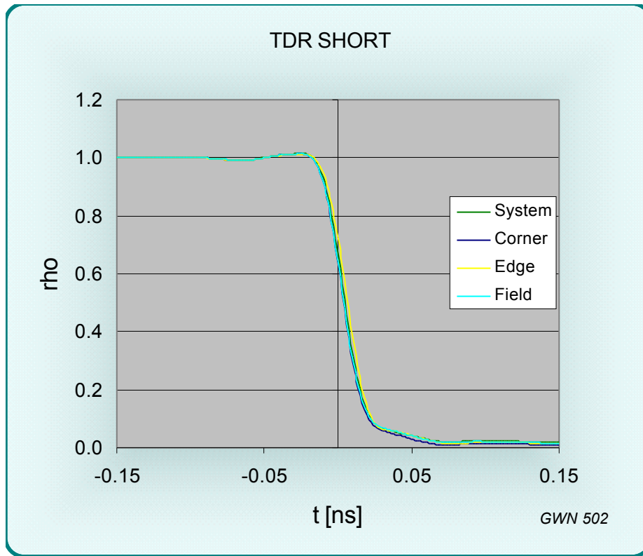
Figure 6 TDR signal from a SHORT circuited DUT test socket
