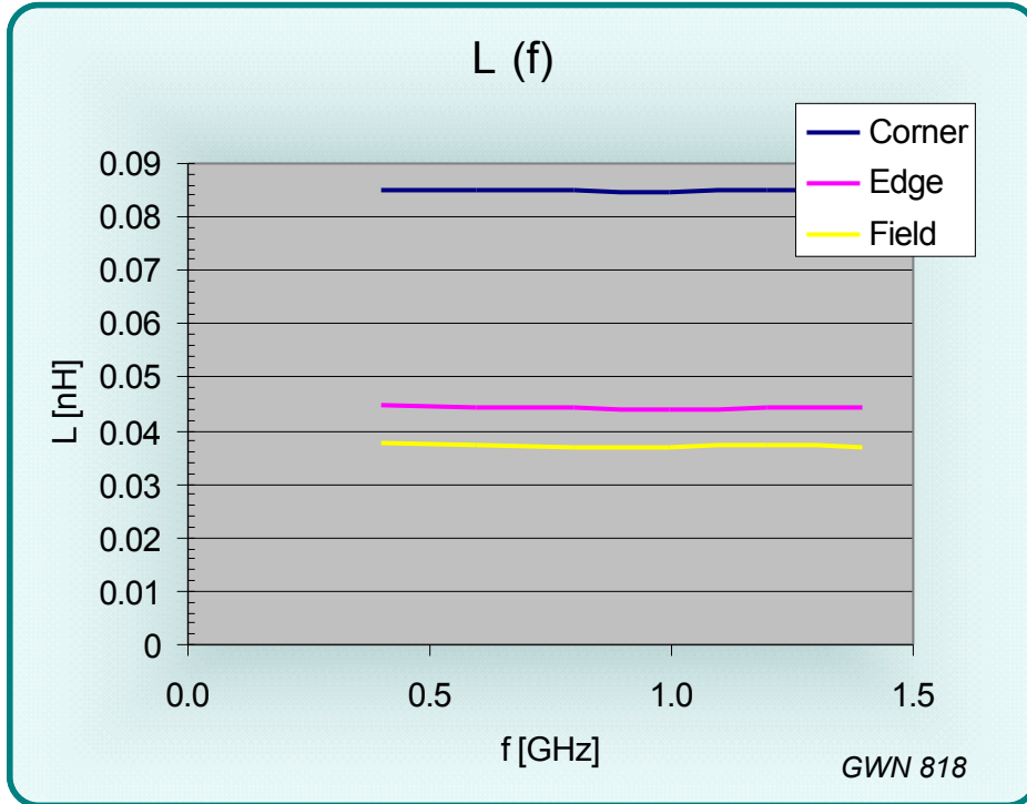
Figure 15 L(f) for the DUT test socket
